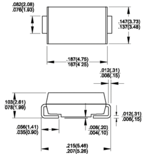
DO-214AA (SMB)
