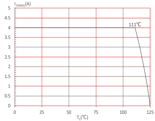
FIG.4: On-state characteristics
