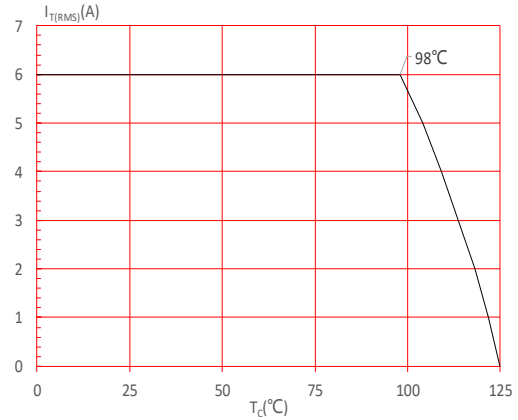
FIG.4: On-state characteristics
