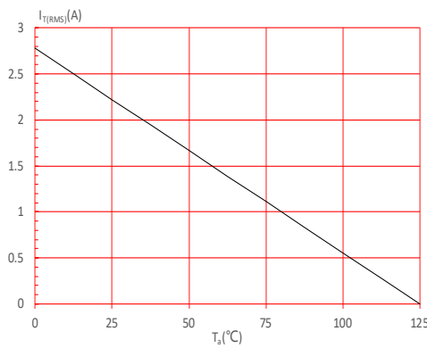
FIG.5: On-state characteristics
