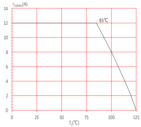
FIG.4: On-state characteristics
