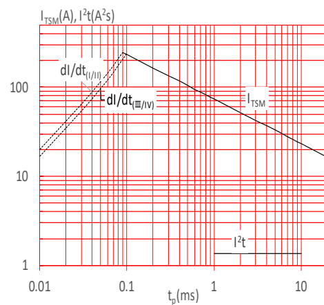
FIG.6: Non-repetitive surge peak on-state current for a sinusoidal pulse with width t_p < 20\text{ms} , and corresponding value of I^2t (I - II: di/dt < 30\text{A}/\mu\text{s} ; III-IV: di/dt < 20\text{A}/\mu\text{s} )
