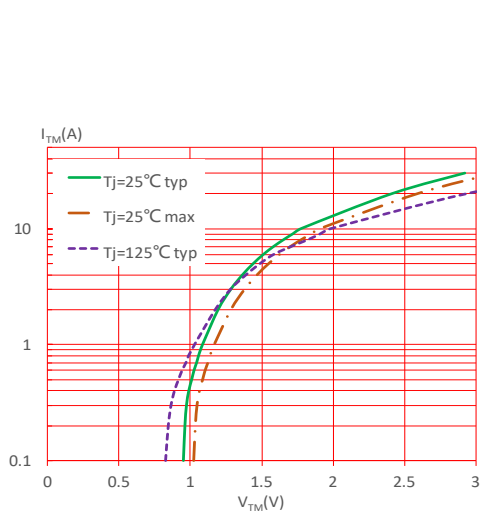
FIG.5: On-state characteristics
