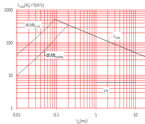
FIG.6: Non-repetitive surge peak on-state current for a sinusoidal pulse with width t_p < 20\text{ms} , and corresponding value of I^2t ( I - II : di/dt < 50\text{A}/\mu\text{s} ; III-IV : di/dt < 30\text{A}/\mu\text{s} )
