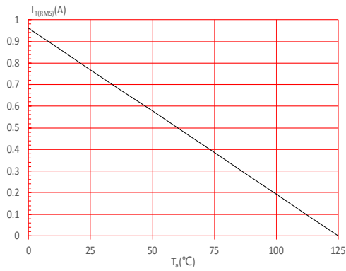
FIG.5: On-state characteristics
