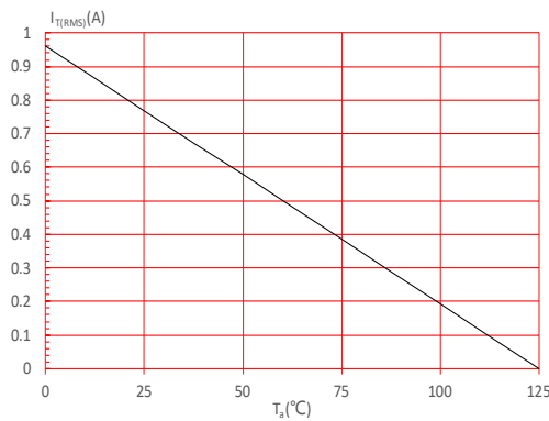
FIG.5: On-state characteristics
