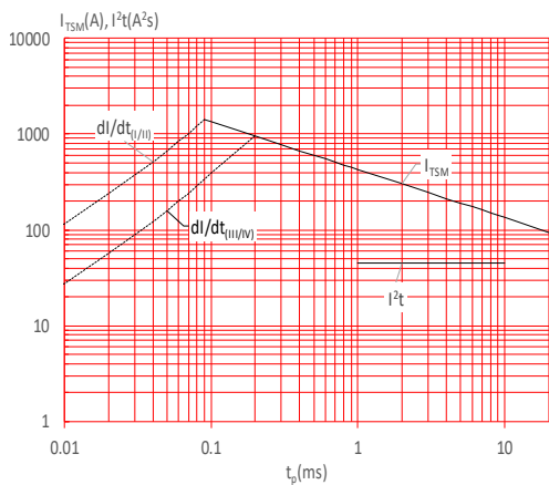
FIG.5: Non-repetitive surge peak on-state current for a sinusoidal pulse with width t_p < 20\text{ms} , and corresponding value of I^2t ( I - II : di/dt < 80\text{A}/\mu\text{s} ; III-IV : di/dt < 50\text{A}/\mu\text{s} )
