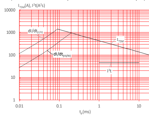
FIG.6: Non-repetitive surge peak on-state current for a sinusoidal pulse with width t_p < 20\text{ms} , and corresponding value of I^2t ( I - II : di/dt < 50\text{A}/\mu\text{s} ; III-IV : di/dt < 20\text{A}/\mu\text{s} )
