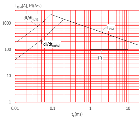
FIG.5: Non-repetitive surge peak on-state current for a sinusoidal pulse with width t_p < 20\text{ms} , and corresponding value of I^2t ( I - II: di/dt < 80\text{A}/\mu\text{s} ; III-IV: di/dt < 50\text{A}/\mu\text{s} )
