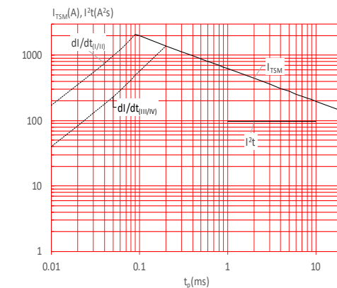
FIG.6: Non-repetitive surge peak on-state current for a sinusoidal pulse with width t_p < 20\text{ms} , and corresponding value of I^2t ( I - II : di/dt < 80\text{A}/\mu\text{s} ; III-IV : di/dt < 50\text{A}/\mu\text{s} )
