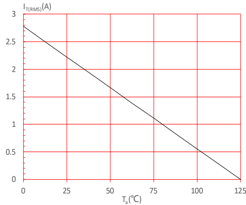
FIG.5: On-state characteristics
