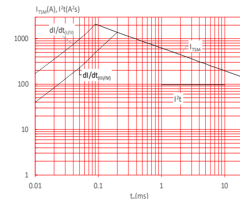
FIG.6: Non-repetitive surge peak on-state current for a sinusoidal pulse with width t_p < 20\text{ms} , and corresponding value of I^2t ( I - II : di/dt < 80\text{A}/\mu\text{s} ; III-IV : di/dt < 50\text{A}/\mu\text{s} )
