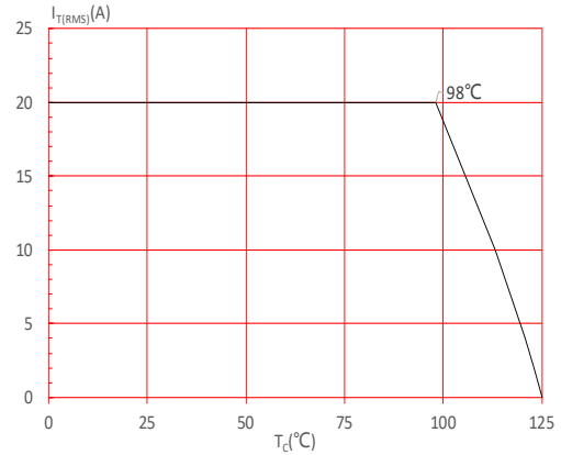
FIG.4: On-state characteristics
