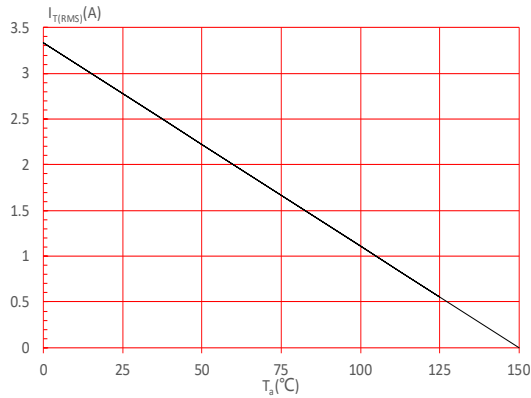
FIG.5: On-state characteristics
