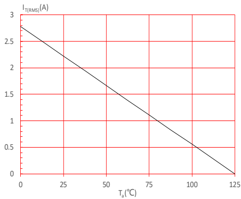
FIG.5: On-state characteristics
