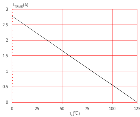
FIG.5: On-state characteristics
