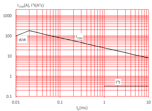
FIG.6: Non-repetitive surge peak on-state current for a sinusoidal pulse with width t_p < 10ms, and corresponding value of I^2t (di/dt < 50A/µs)
